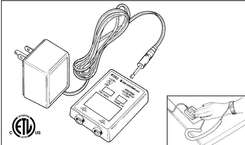
Figure 1. Model 41193 Wrist Strap Touch Tester / Common Point Ground
