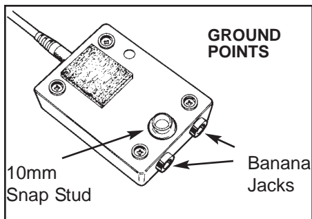
Figure 6. Ground points.
