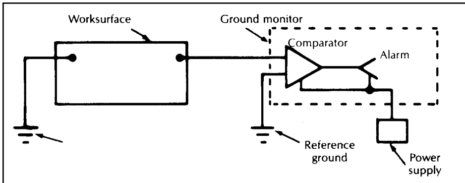
Figure 6. Block diagram of a ground-integrity monitor.
