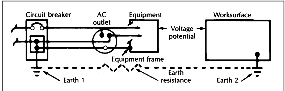
Figure 2. Separate ground systems present potential problems.
