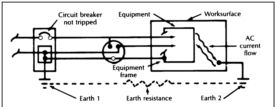
Figure 3. How current flow through a work surface is generated.
