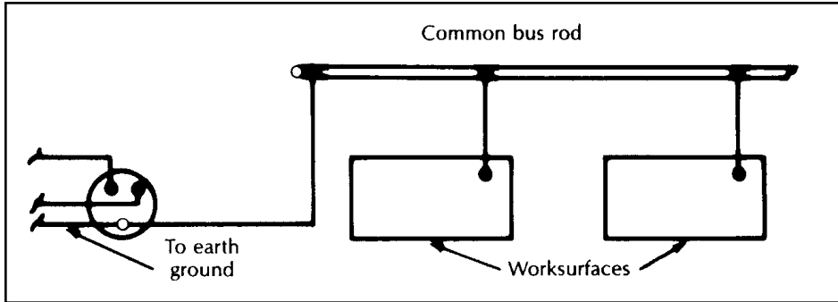
Figure 5. Grounding strategy for workstations without AC power.
