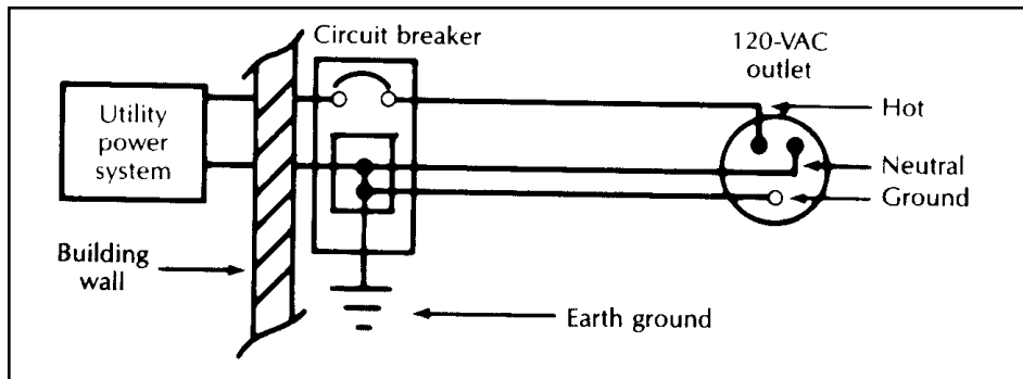
Figure 1. Earth grounding in a typical 120-V, 60-Hz electrical system
