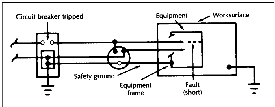
Figure 4. The relationship between equipment (or safety) ground and earth ground.
